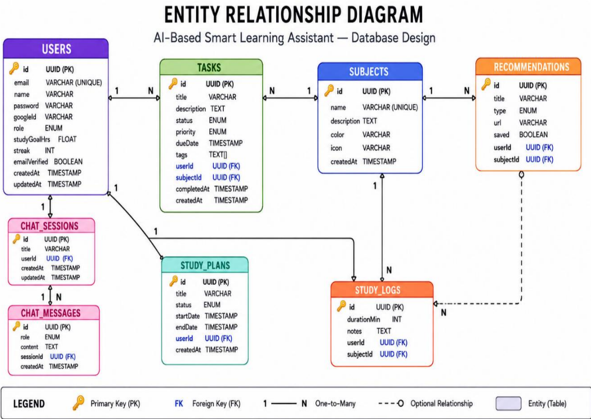
Figure: Entity Relationship (ER) Diagram of the AI-Based Smart Learning Assistant
